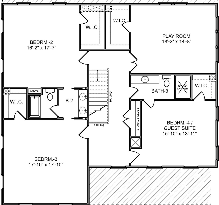
UPPER LEVEL PLAN
